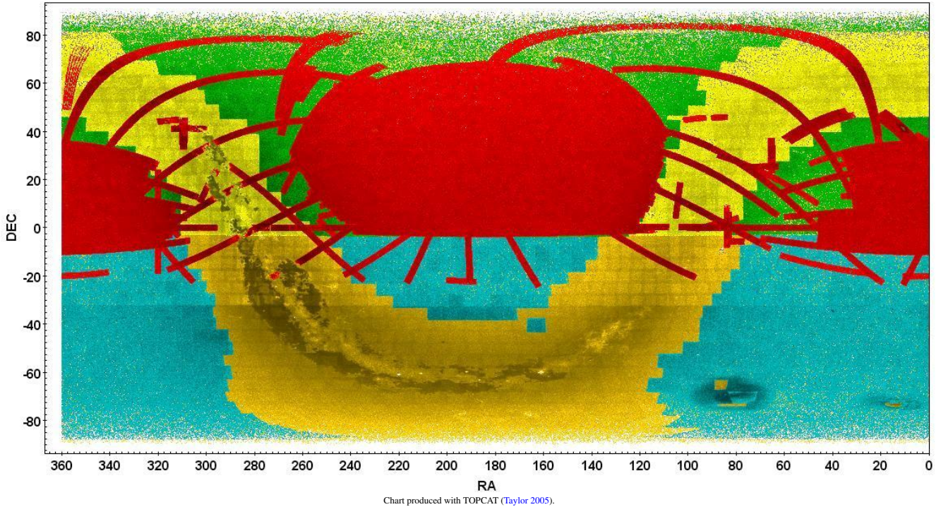
Figure 1. Sky coverage of the ASP catalogue, using 1% of the data. Stellar density shows as grey background (compare Figure 3). Colours designate catalogue/survey photometry coverage as follows:
