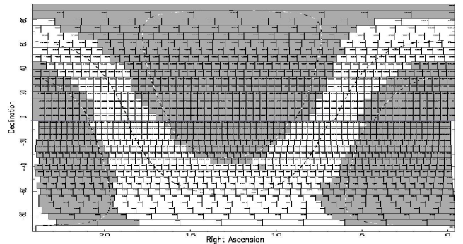
Figure 2. APM sky coverage: dark areas.
