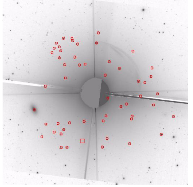
Figure 4. Sky around the star 31 Leo (J100754.3+095951) from a 12 arcmin-sq SDSS finding chart. Red circled objects appear in ASP with epoch-1955 POSS-I astrometry from the APM & USNO-A catalogues; they ring the masked central star because neither the SDSS nor USNO-B catalogues identified them in the glare of the central star. Objects farther out than 4.5 arcminutes’ radius from the central star are reported with astrometry of later epochs from SDSS and USNO-B. At J100757.9+095617, shown as a large red square at lower left, a stellar object of R=18.3 appears on the POSS-I plates but is not seen at later epochs.
