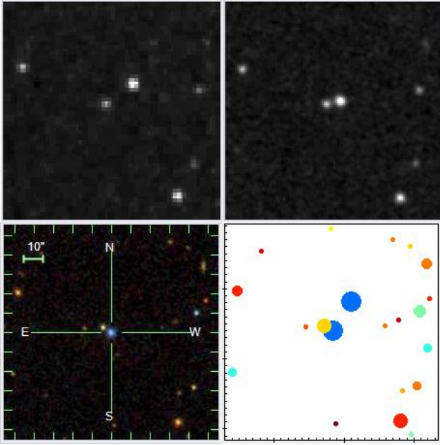
Figure 5. The white dwarf SDSS J090514.79+090426.2 across the epochs, all images are 2' \times 2' and centred on the SDSS position. Upper left: POSS-I red plate from the 1950's; upper right: POSS-II red plate from the 1980's; lower left: SDSS chart from the 2000's. Star shows proper motion with bearing of 147^\circ E of N. Lower right: this sky as represented in ASP: disk sizes represent V magnitude, red-blue colours using a rainbow palette. The white dwarf star is present twice, once at the SDSS position at centre, and once at the POSS-I position which is flagged with epoch 1955. ASP does flag the object at centre as showing proper motion – flag taken from USNO-B.
