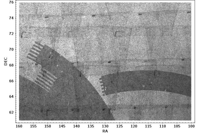
Figure 7. Northern high-latitude sky density. The edge of the main SDSS footprint and an SDSS extension arc are seen across the bottom half. APM & USNO-B POSS-I plates (with thin margins and small USNO-B label artefact at their upper left corners) and USNO-B POSS-II plates (with broad margins and label edge artefact at their lower right corners) are seen to overlap differentially as they near the pole.
