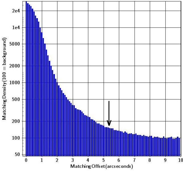
Figure A4. Many-to-one matching of full POSS-I Schmidt plate data with neighbouring plates with narrow overlaps (see depiction on Figure 6), binned to annuli of 1/10th arcsecond width; n = 436\,832 matches over 83 two-plate overlaps. The priority here was to remove duplicates, more importantly than retaining close doublets. Therefore the desired matching radius was farther out than the ( y=200 ) crossing point which here is at x=4.45 . I selected 5.35 arcseconds simply to be consistent with other matchings, shown by the arrow. The unremoved duplicates in the area x > 5.35 and y > 100 comprise a residue which can reach large offsets because systematic offsets at plate edges can point oppositely to that of overlapping plates.
