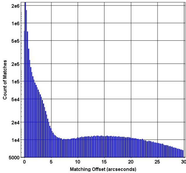
Figure A1. One-to-one matching of SDSS data to APM/USNO-B combined data, binned to annuli of 1/5^{th} arcsecond width. The vertical scale is logarithmic to improve visibility at low counts, n = 8\,733\,411 matches for this chart.
