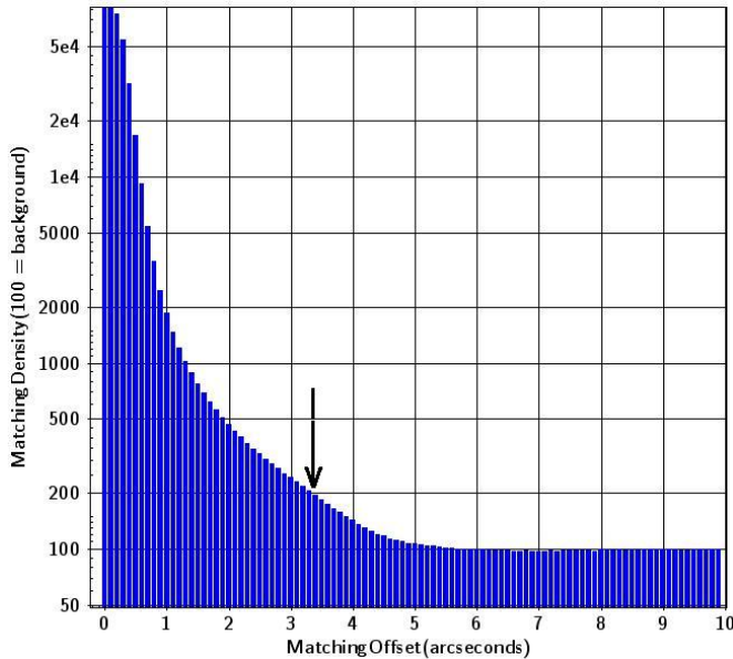
Figure A2. Many-to-one matching of SDSS data to APM/USNO-B combined data, binned to annuli of 1/10^{th} arcsecond width. The vertical scale is logarithmic to improve visibility at low counts; n = 11\,567\,232 matches over 1170 sq degrees for this chart. The background density is normalized to y=100 ; therefore, the chart area below the line y=100 represents the true background of discrete objects, with chart area above y=100 representing duplicates. The arrow shows where the profile crosses the y=200 line – there, at x=3.35 , the count of duplicates equals the background count of discrete objects.
