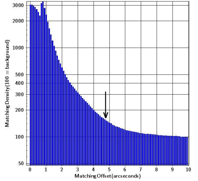
Figure A5. Many-to-one matching of multi-catalogue POSS-I data against attenuated* USNO-B POSS-II data, binned to annuli of 1/10th arcsecond width; n = 10\,880\,162 matches over about 8000 sq degrees of sky. The priority here was to remove duplicates, but there was increased scope for retaining true objects from each survey which had no counterpart in the other survey. There was no absolute answer in choosing the matching radius, so I chose a midpoint between the usual value of 5.35 and the y=200 crossing at x=4.0 ; thus, I decided on 4.75 arcseconds as the matching radius, indicated by the arrow. The double peak at x=0 , x=0.7 is because USNO-B data granularity is 0.7 arcsec, so matches closer than that are to APM or USNO-A data, and the peak at x=0.7 arcsec is largely from adjacent USNO-B data.
