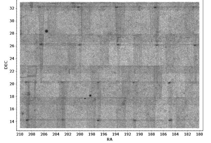
Figure 6. Northern Galactic Cap sky density tile with SDSS objects removed, darker is denser. Two photographic plate grids are seen: POSS-I plates with thin overlaps are arrayed at 6^\circ intervals and show a small USNO-B artefact of spurious data at the upper left corner of each plate, probably from a rectangular label. POSS-II plates constitute another lattice and are seen throughout with broad overlaps arrayed at 5^\circ intervals. Overlap zones are denser because of unique data contributed by each plate, plus some far-offset duplicates.
