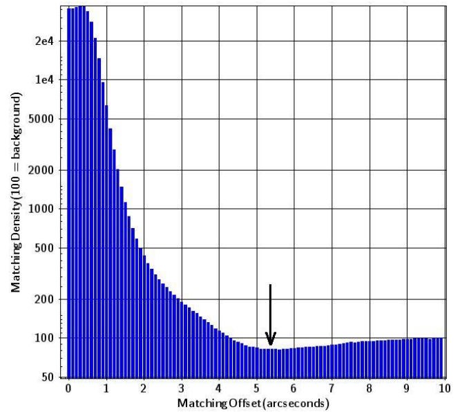
Figure A3. Many-to-one matching of APM to USNO-B data in the UKST survey area, binned to annuli of 1/10^{th} arcsecond width with logarithmic vertical scale; n = 11\,731\,786 matches from 50 Schmidt plates for this chart. The profile is hollowed out below background from x=4.4 to 9. This appears to be because APM reports objects closer to bright stars than does USNO-B, see e.g., Figure 4; in matching them, this simulates an internal edge effect within USNO-B data because true objects are missing across the edges of the effective holes, thus lowering matching rates below background. The matching radius was set at the inflection point of 5.35 arcseconds (indicated by the arrow) in tandem with the radius used for the POSS-I data which has a similar profile.
